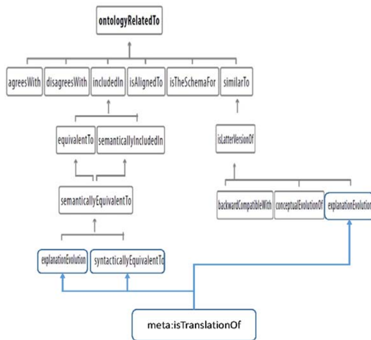
Fig. 2. Extension of DOOR ontology.
